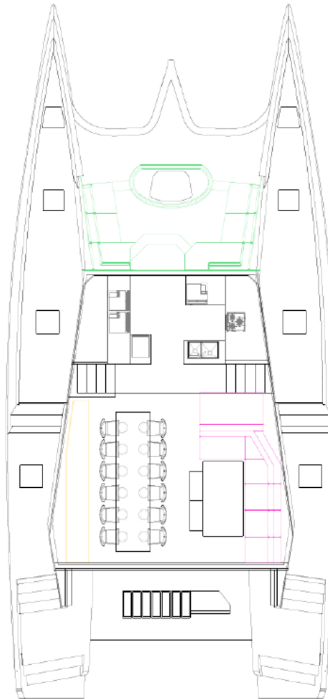
DAY CHARTER VERSION - WITH GALLEY FORWARD & LARGE DINING ROOM, STANDARD 3 CABIN LAYOUT IN HULL.
