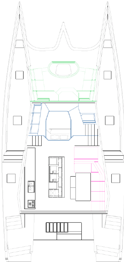
MAIN DECK MASTER VERSION - WITH CREW CABIN AND UTILITY ROOM.
